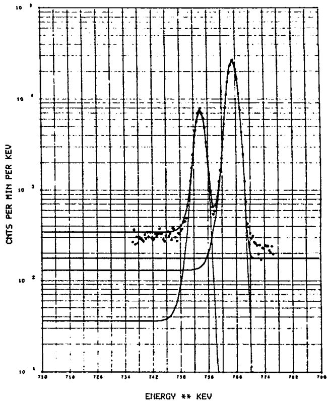
Fig. 401-5. The fitted spectra for the ^{95}\text{Zr} 756 keV and ^{95}\text{Nb} 765 keV gamma-ray peaks.
