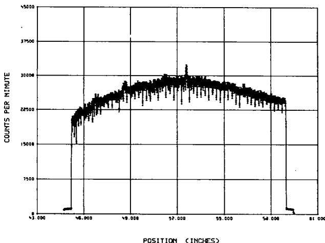
Fig. 401-7. The ^{95}\text{Zr} axial isotopic distribution of a failed mixed-oxide fuel pin.
